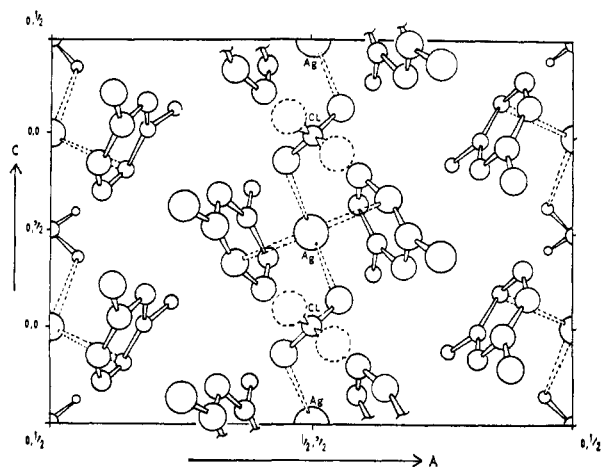
Figure 1. A perspective view of the (m\text{-xylene})_2 \cdot \text{AgClO}_4 structure down the b axis. The Ag and Cl atoms lie on crystallographic twofold axes normal to the plane of the paper. The distorted tetrahedral arrangement about Ag is made up of oxygens from two \text{ClO}_4^- ions and carbons from two m -xylene molecules.
