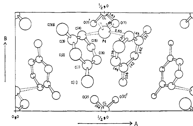
Figure 2. A perspective view of the (m\text{-xylene})_2 \cdot \text{AgClO}_4 structure down the c axis. The \text{AgClO}_4 "sheet" is at a/2 , and the \text{AgClO}_4 chain propagates normal to the plane of the paper.
